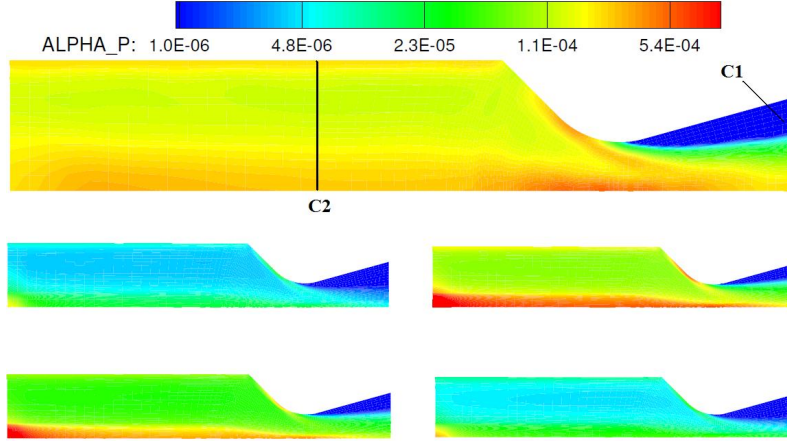
Figure 5: Instantaneous volume fraction : Lagrangian (Top) and Sections (Bottom : Sect. 1 (1,1), Sect. 2 (2,1), Sect. 3 (1,2) and Sect. 4 (2,2)).
