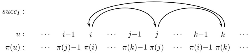
Fig. 2.3: Illustration of the equivalence I \sim \pi on three integers (i, j, k) such that j = \text{succ}_I(i) and k = \text{succ}_I(j) . It can be checked that \pi(v) = \pi(u - 1) + 1 for any (u, v) \in \{(i, j), (j, k), (k, i)\} .
