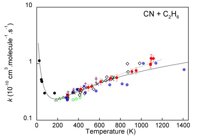
FIG. 6: Rate coefficients for the reaction of CN( X^2\Sigma^+ ) with ethane, C 2 H 6 , as a function of temperature. This work: (●). Yang et al. [28] between 185 and 739 K: (△). Hess [29] over the 294–736 K range: (×). Herbert et al. [30] over 297–694 K range: (+). Balla et al. [31] using PLP-LIF and diode absorption spectroscopy over the 292–1409 K: (⊕). Copeland et al. [32] over the 279–452 K range: (★). Atakan et al. [33] over the 294–984 K: (◇). Bullock et al. [34] over the 300–415 K range: (◊). Sims et al. using a supersonic uniform flow reactor (CRESU) [35]: (●). The full line represents theoretical calculations by Georgievskii and Klippenstein [36] over the 20–1140 K range combining VRC-TST and 2TS. The dotted line correspond to the fit of our data over the 298–1116 K range.
