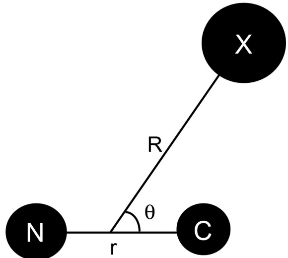
FIG. 8: Coordinate system of the \text{CN} - \text{X} ( \text{X} = \text{He}, \text{Ar} ) complex.
