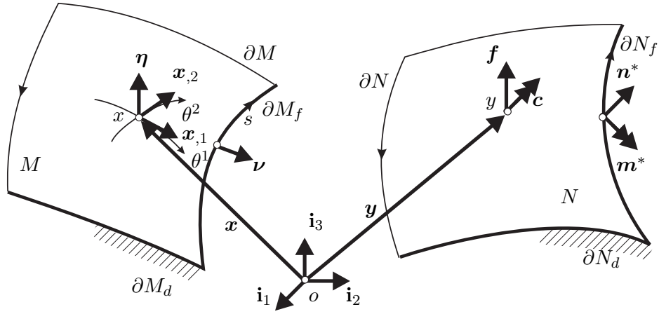
FIG. 1. Shell kinematics.
