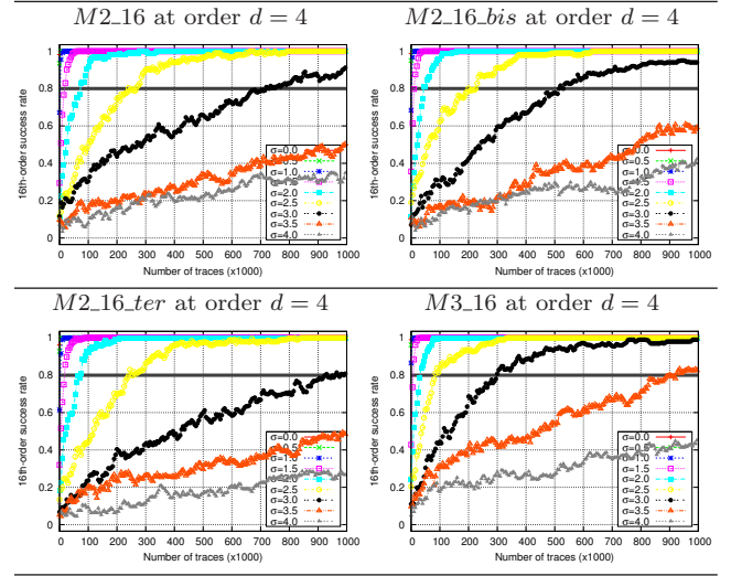
Figure 2: 16th-order success rates for 4th-order CPA for \sigma \in \{0, \frac{1}{2}, 1, \dots, 4\} , and a budget of 1 million traces.
