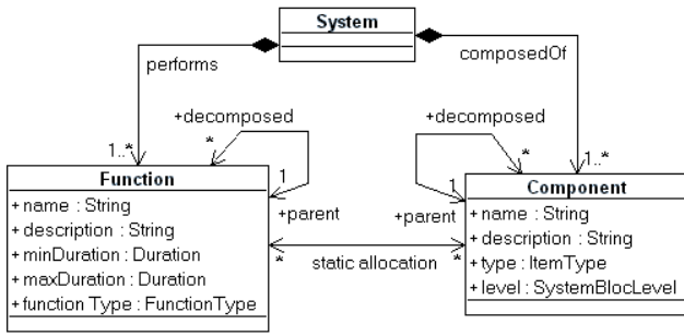
Fig. 2. Part of the meta-model defined in [1]
