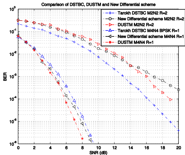
Figure 1. Simulation results of DSTBC [7] [9], DUSTM [6] and our new differential space-time modulation scheme.
