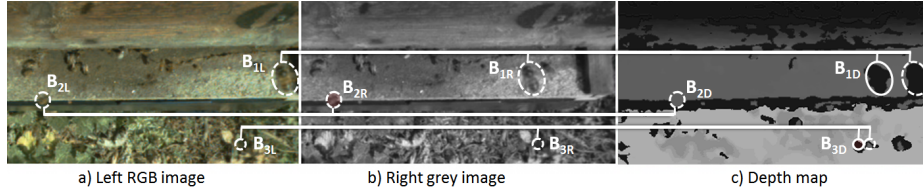
Fig. 5. Different depth map effects observed with the G3 EV camera. B 1 (high speed target) isn't matched between a) and c), and it results in the right shadow effect on c), plus its high height from the background produces the additional left shadow effect. B 2 (non moving target) is correctly matched but being closed the background, no shadow effect is observed. B 3 (normal speed target) is half matched and produces a double shadow effect for the same reasons as B 1
