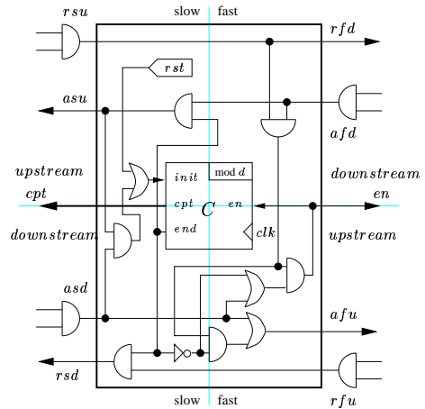
Figure 7. Control Unit
