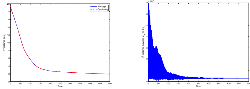
Figure 3: H^s norm to the ground state (left) for the averaged system (continuous line) and the oscillating system (dashed line). H^2 gap from the average (right).
