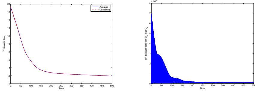
Figure 4: H^s norm to the ground state (left) for the averaged system (continuous line) and the oscillating system (dashed line). H^2 gap from the average (right).
