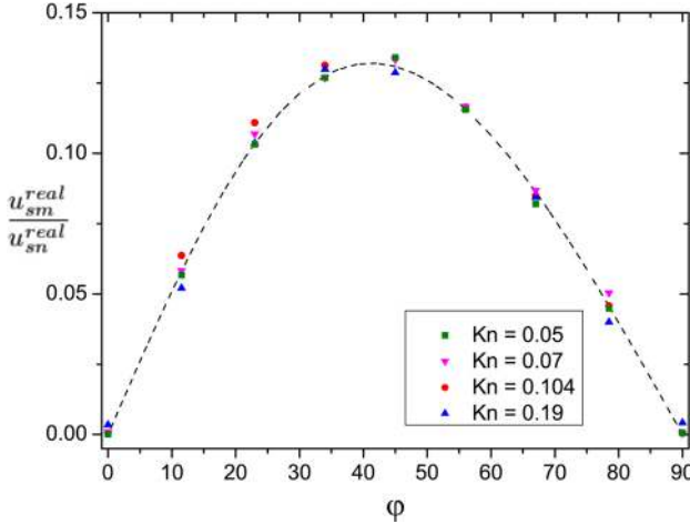
Fig. 8 Ratio of transverse and longitudinal components of real slip velocity as a function of \varphi for different Kn. Points are MD data and the dashed line is for the analytical expression (33).
