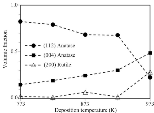
Figure 10 Distribution as a function of deposition temperature of (001)- and (112)-oriented anatase and (100)-oriented rutile crystallites for TiO 2 films grown on C-plane sapphire.
