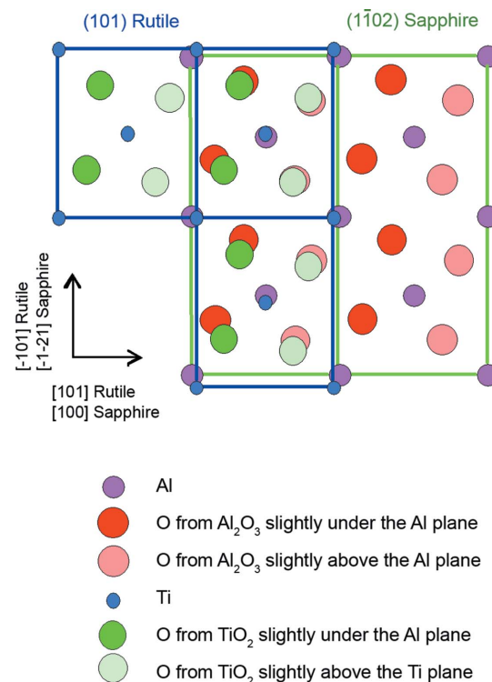
Figure 11 A sketch of the atomic coincidences at the interface between (101) rutile and (1\bar{1}02) sapphire. For clarity, three unit cells of rutile and two of sapphire are drawn and the atom sizes are not scaled.
