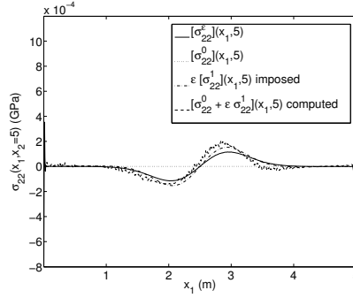
Figure 12: Exemple 2 ( \epsilon = 0.01 m) – Jump in the stress [\sigma_{22}](x_1, x_2 = 5) (GPa) along the interface
