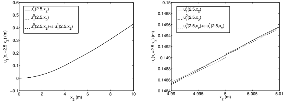
Figure 13: Exemple 2 ( \epsilon = 0.01 m) – Displacement u_1(x_1 = 2.5, x_2) (m) on a vertical cut (Zoom on the right)
