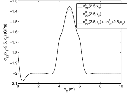
Figure 11: Exemple 2 ( \epsilon = 0.01 m) – Stress \sigma_{22}(x_1 = 2.5, x_2) (GPa) on a vertical cut
