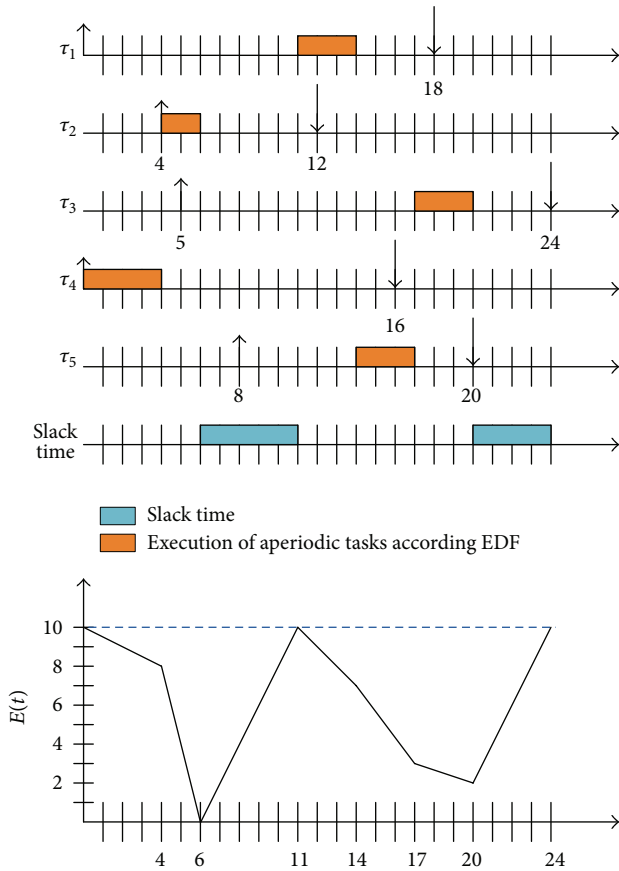
FIGURE 4: Example on EH-EDF scheduling.
