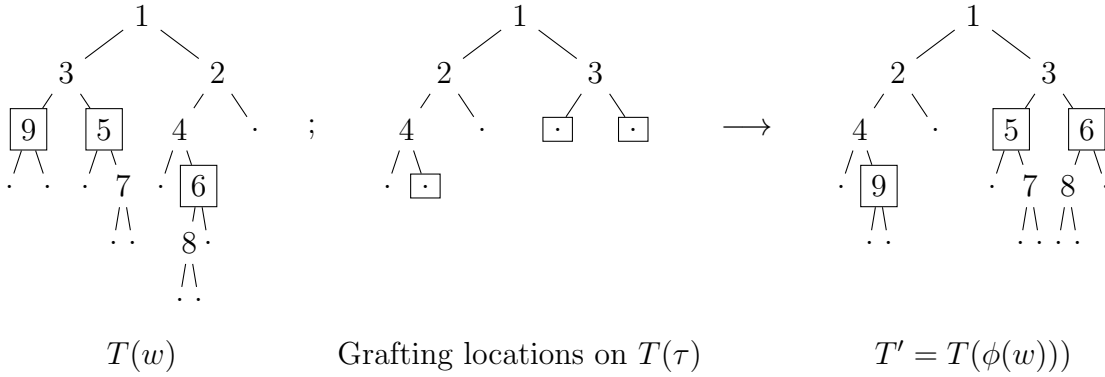
Figure 4: Construction of T' with \sigma = 3142 , \tau = 4213 , s = 51342 , and w = 935714862 .
