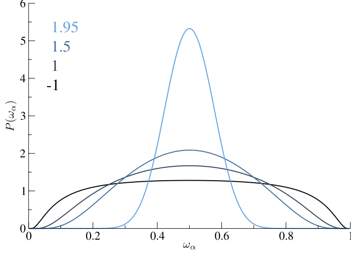
Figure 5. The distribution P(\omega_\alpha) in equation (7.11) for different \alpha < 2 in 2D systems.
