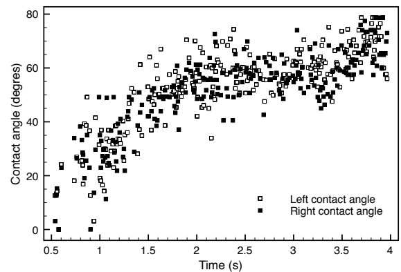
Figure 6: Evolution of the left and right contact angle of the macro-drop with time. Data are plotted for 'R' test.
