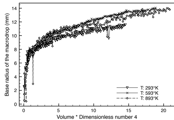
Figure 10: Evolution of the base radius of the macrodrop in relation with mass transfert and energy effects. Dimensionless number 4: \pi_4 = \frac{Ppc_p^{1,5}}{\lambda^2 \sqrt{\Delta T}} . Data are plotted for 'T' tests.
