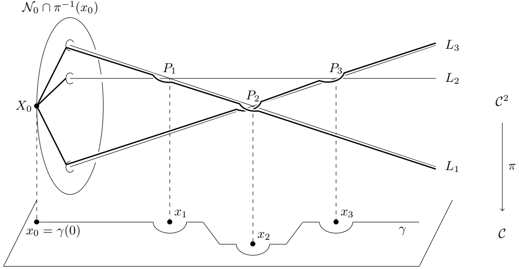
FIGURE 5. Construction of \delta(\varepsilon)
