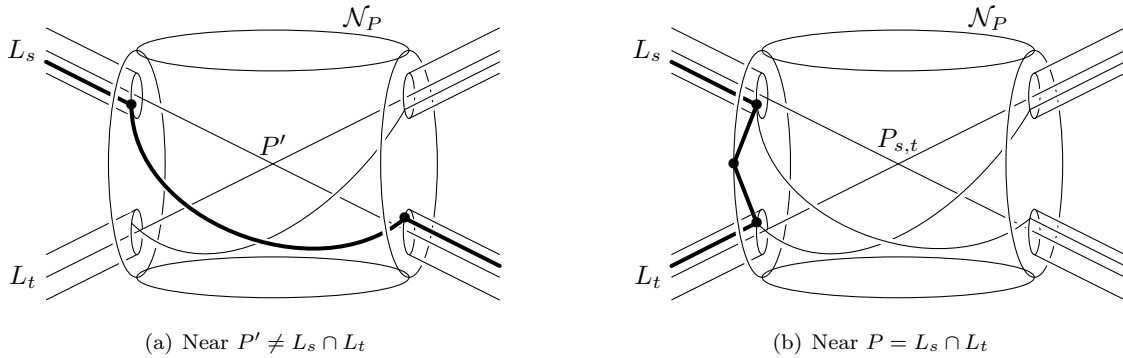
FIGURE 4. Construction of \varepsilon_{s,t} near singular points.
