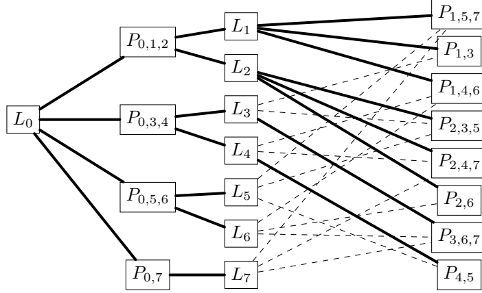
FIGURE 7. Incidence graph of MacLane's arrangement Q^+
