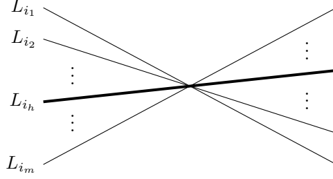
FIGURE 6. Indexation of a crossing
