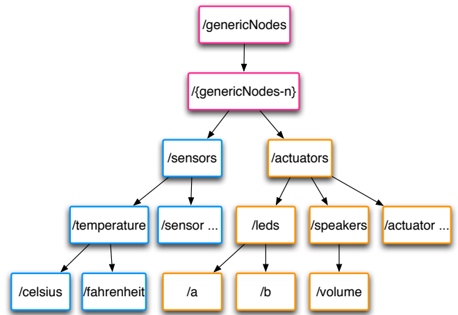
Fig. 2. Resource hierarchy example of an abstract node
