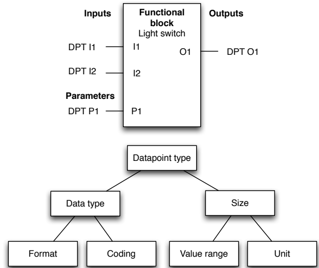
Fig. 4. Functional block structure and datapoint type composition
