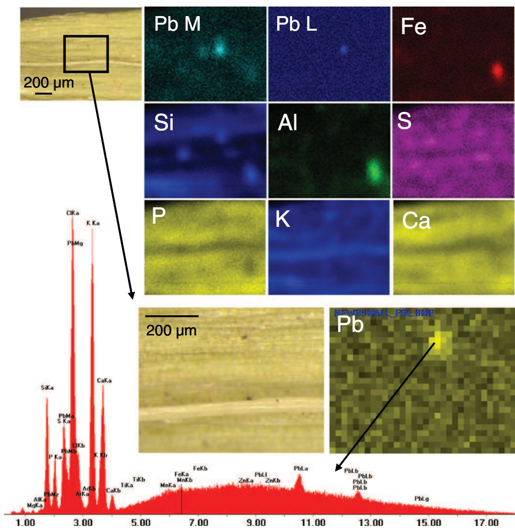
Fig. 2. \mu XRF elemental maps obtained for a portion of ryegrass leaf, and \mu XRF spectrum of the Pb-rich spot.
