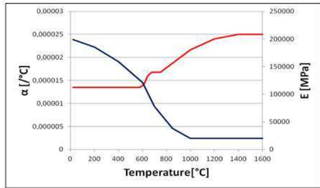
Fig. 5 15-5 PH Young modulus and expansion coefficient
