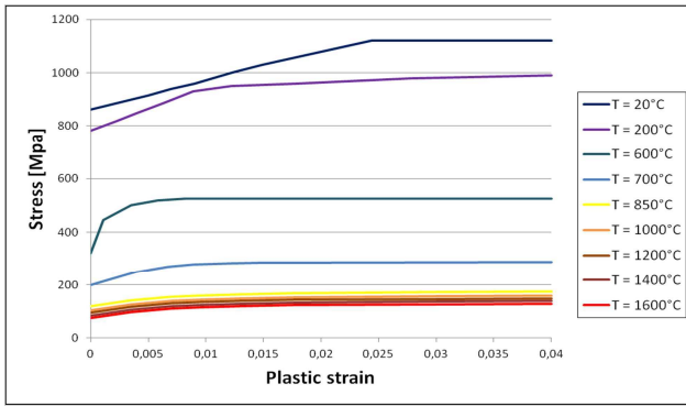
Fig. 4 15-5 PH Hardening curves
