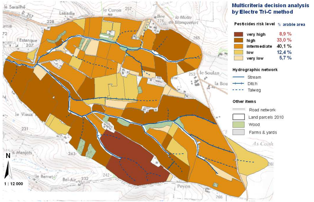
Fig. 7- Auradé Watershed: spatialised results of MCDA modelling for pesticides, with effect of BEPs
