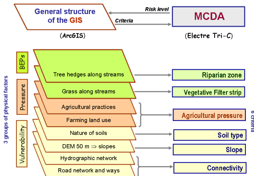
Fig. 6- Various criteria analysed for the assessment of pesticide risks and the BEPs effects
