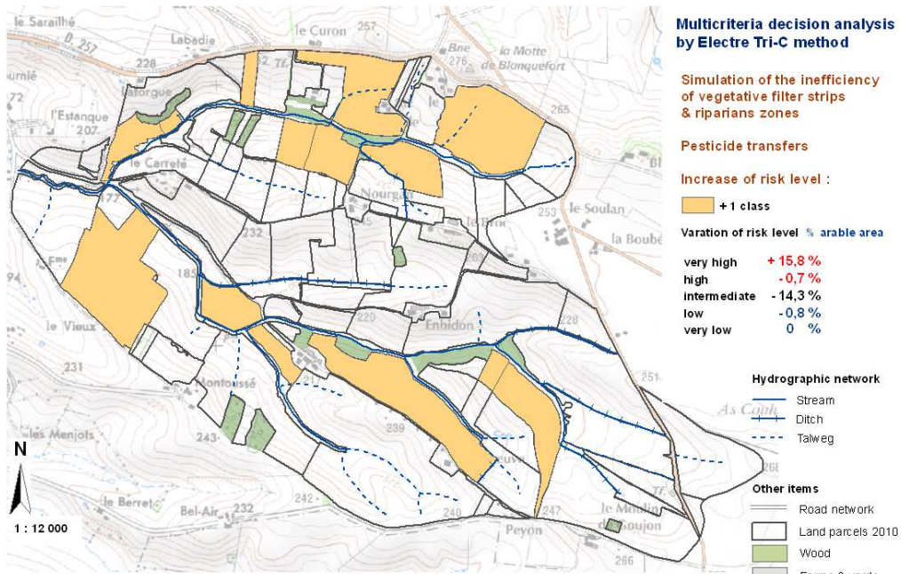
Fig.8- Auradé Watershed: agricultural parcels with a risk increase, without any BEPs effect
