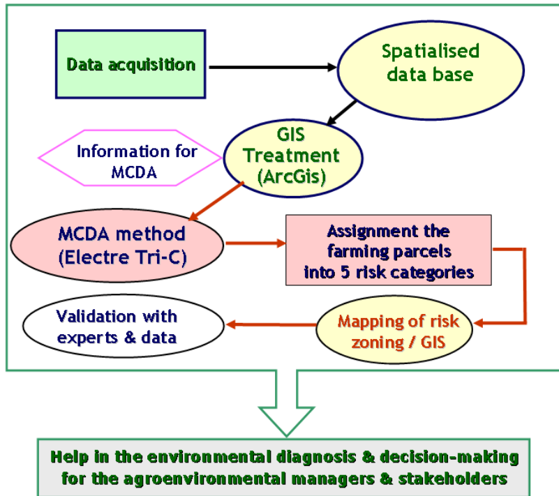
Fig. 5- General diagram of the method combining GIS and MCDA
