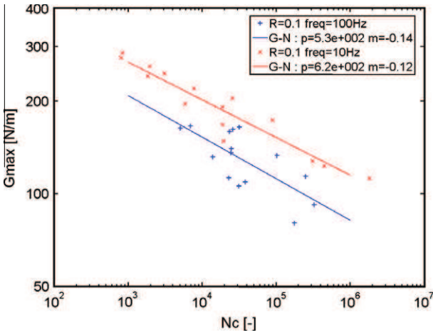
Fig. 14. G-N propagation curve: 10 Hz and 100 Hz.
