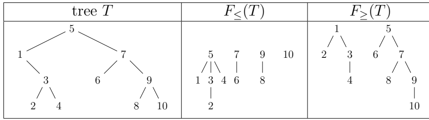
FIGURE 4. A tree with its increasing and decreasing forests.
