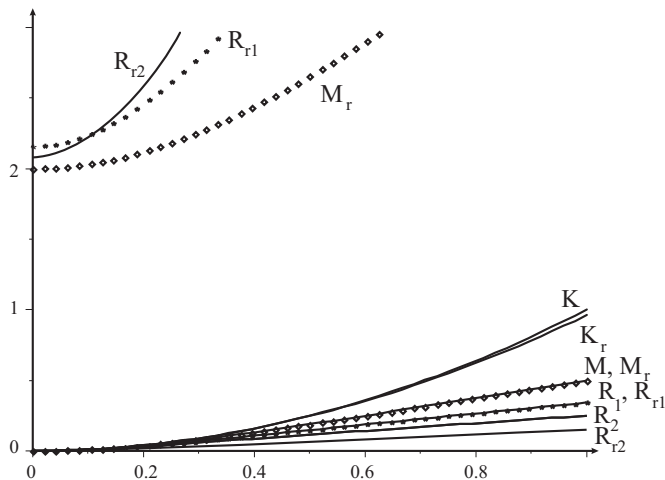
Figure 5: Dispersion curves: K – Kirchhoff plate; M – Mindlin plate; R_1 and R_2 – Reissner sandwich plates with h_f = 0.1h , \alpha = 0.1 , and h_f = 0.05h , \alpha = 0.05 , respectively. K_r , M_r , R_{r1} , and R_{r2} are the corresponding dispersion curves with taking into account the rotatory inertia
