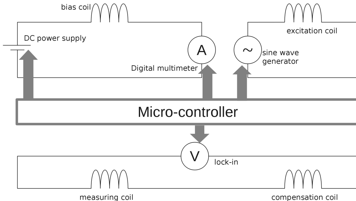
Figure 3 : set-up controller
