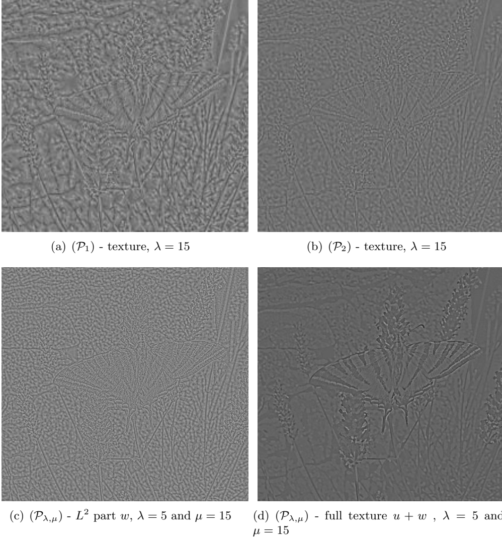
Figure 3.29: Comparison for texture extraction. The textures in (\mathcal{P}_1) and (\mathcal{P}_2) are defined as the remainder term “data - solution”. The texture in (\mathcal{P}_{\lambda,\mu}) is defined as w and we present u + w as well.
