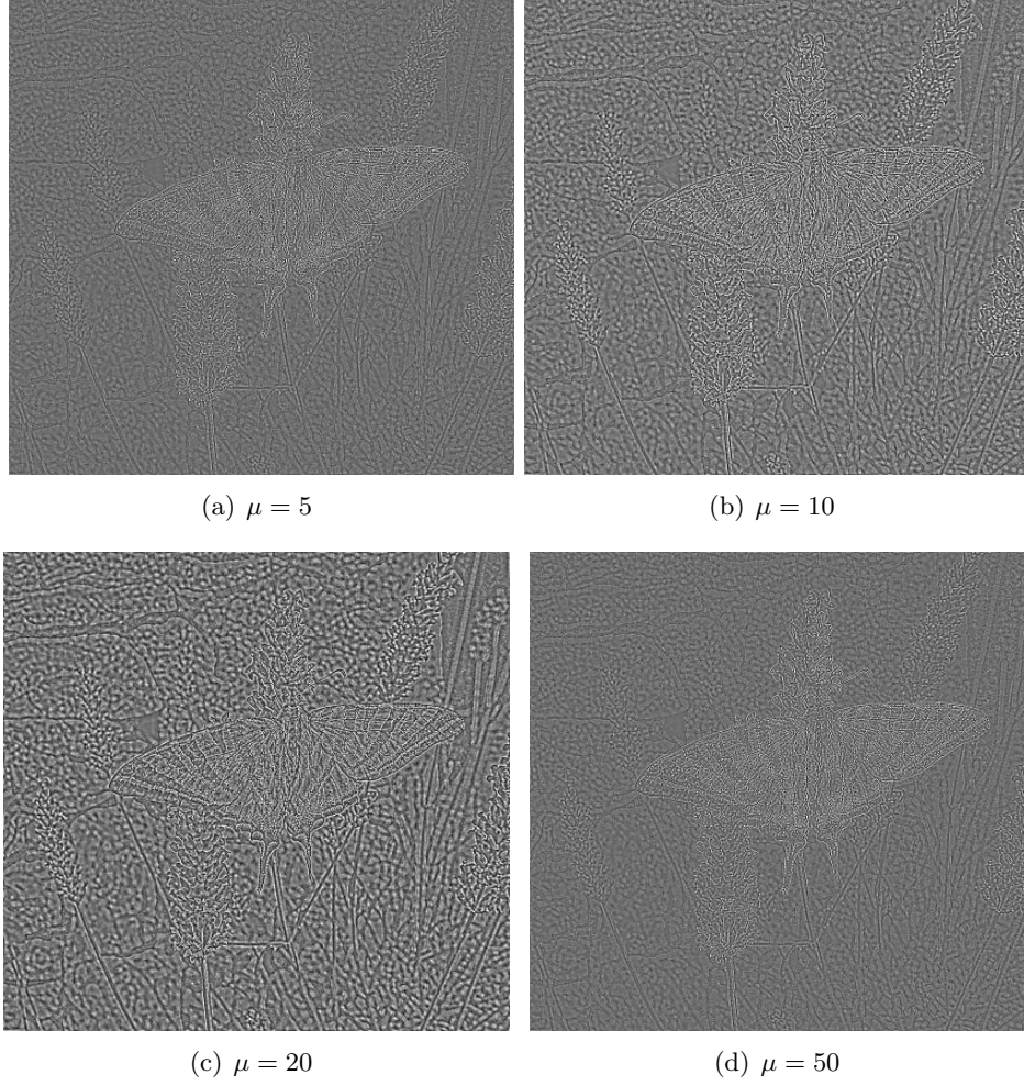
Figure 3.25: L^2 component - w = u_d - u - v - \lambda = 10
