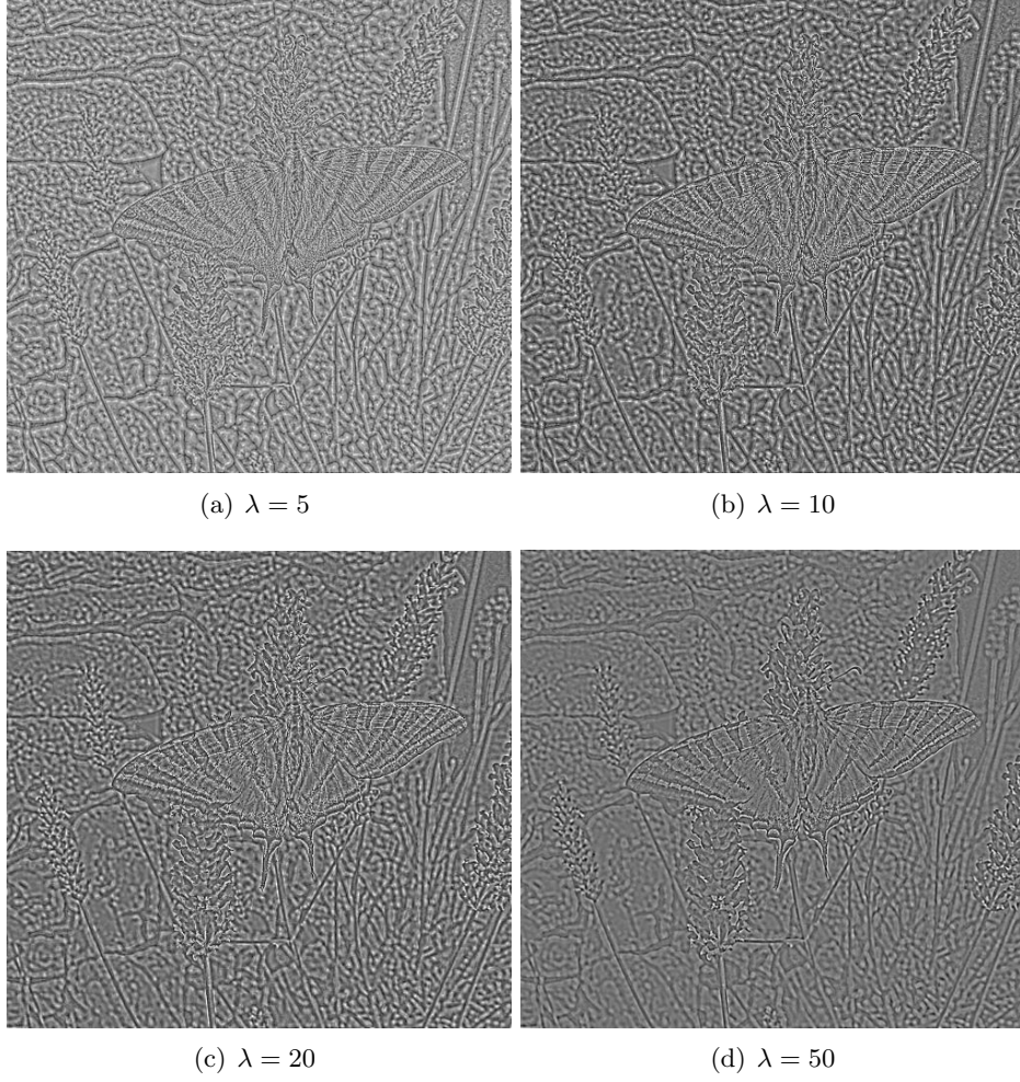
Figure 3.22: L^2 component - w = u_d - u - v - \mu = 50
