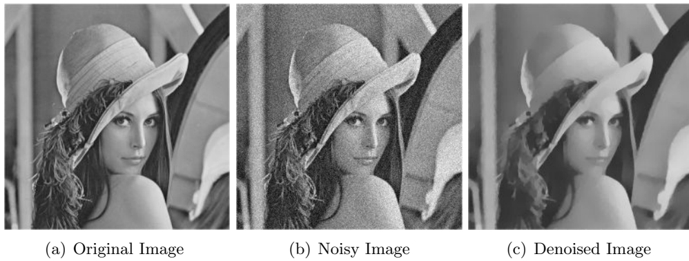
Figure 3.1: ROF denoising process - Gaussian noise with standard deviation \sigma = 0.25 and \lambda=50 . Staircasing effect
