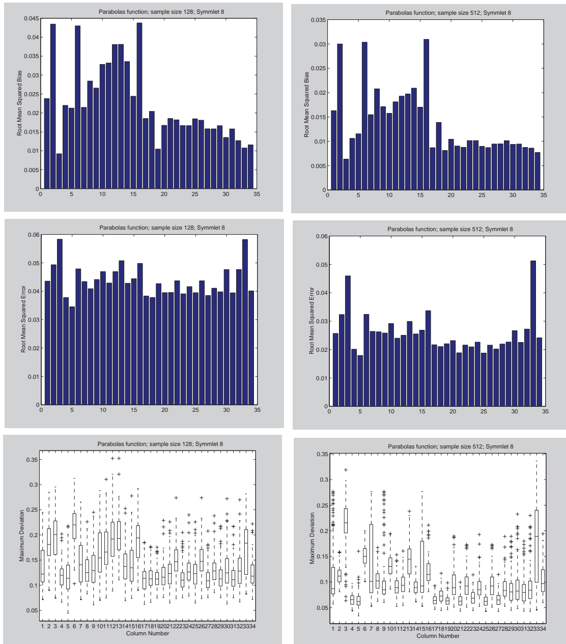
Figure 8.12: Performance of the estimators for the Parabolos function over 100 simulations. The root signal-to-noise ratio is equal to 3 for sample sizes of 128 (left) and 512 (right) design points. The wavelet filter used is the Symmlet 8.
