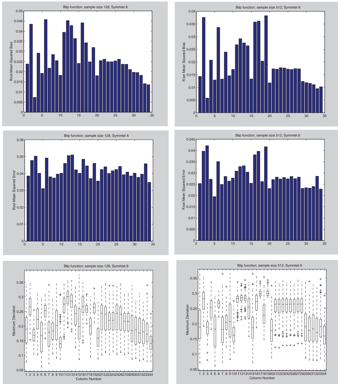
Figure 8.6: Performance of the estimators for the Blip function over 100 simulations. The root signal-to-noise ratio is equal to 3 for sample sizes of 128 (left) and 512 (right) design points. The wavelet filter used is the Symmlet 8.
