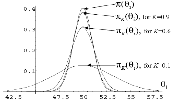
Fig.2. Weighted prior for different values of K
