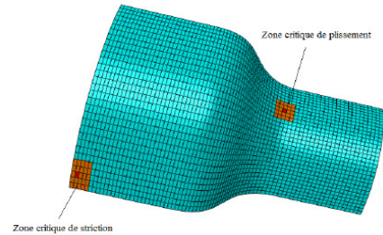
Fig. 7. Localization of the critical elements.
