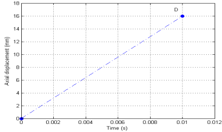
Fig. 3. Loading path: displacement (mm) – time (s).
