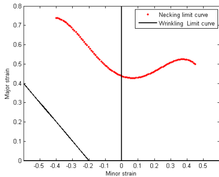
Fig. 6. Forming Limit Curve (FLC).
