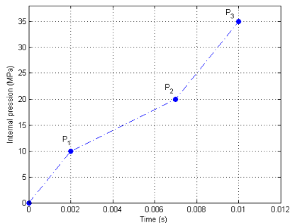
Fig. 4. Load path: pressure (MPa) - time (s).
