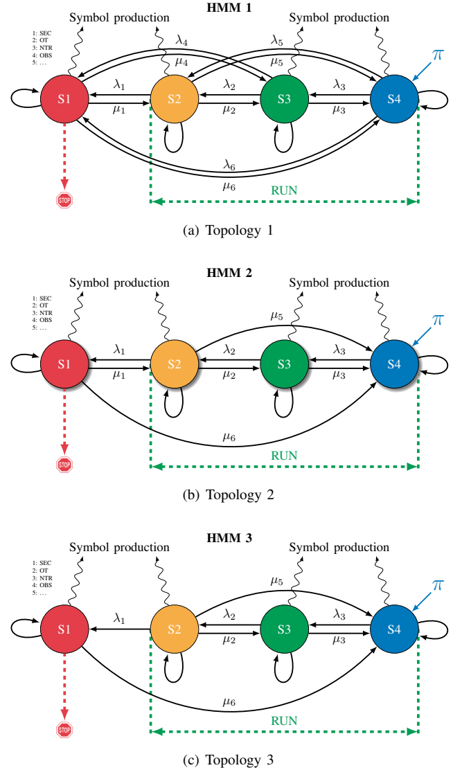
Fig. 1. The four-state Hidden Markov Model. Different topologies are represented. All transitions are permitted on 1(a). In 1(b) and 1(c) we removed some transitions, in order to have a more representative topology that was more representative of an industrial situation. S1 to S4 represent the degradation levels. S1: the system is stopped. S4 to S2: progressive degradations of the process. The production of symbols represents the Markov chain given by a maintenance database. \lambda_i is the failure rate and \mu_i is the repair rate. \pi is the initialization matrix.
