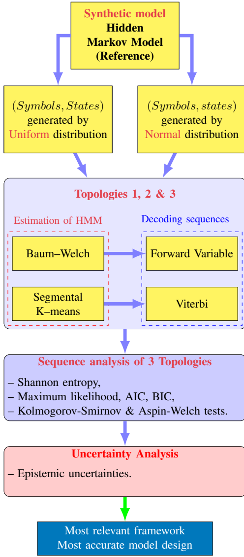
Fig. 3. The matching model method, using a Synthetic Model: We first used the Synthetic Model (also called reference model), to generate stochastic 2-tuple (Symbols, States) by using the Normal and the Uniform distribution. Thus, we injected these signatures into the 3 topologies of Hidden Markov Model. To achieve learning models, we use Baum-Welch learning, decoding by Forward Variable and Segmental K-means learning, decoding by Viterbi. We obtained new sequences of (Symbols, States) that we analyzed. We evaluated the best topology, best learning algorithm and best distribution. To evaluate this "signature", the following widely-used criteria have been applied: Shannon Entropy, Maximum Likelihood, Akaike Information Criterion (AIC), Bayesian Information Criterion (BIC) and Kolmogorov-Smirnov & Aspin-Welch statistical tests. Finally, epistemic uncertainties make it possible to frame the margin error of the model design. The synthesis of all these criteria, yielded the best relevant framework.
