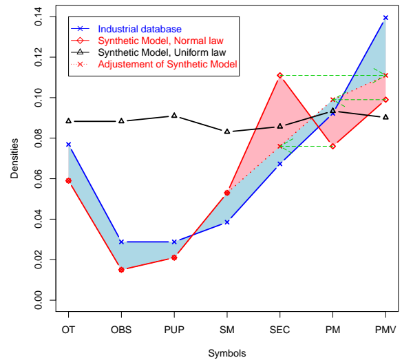
Fig. 4. Densities comparison, between the Synthetic Model and a real maintenance database from a bread production factory. You can see that the Synthetic Model with the Normal distribution, has almost the same shape as the real industrial data. Whereas the Synthetic Model with the Uniform distribution does not follow the industrial shape. We made an adjustment of the Synthetic Model (in red dotted), to have a better correlation coefficient. Green dotted arrows are the proposed changes for the new model. SEC \rightarrow PMV, PM \rightarrow SEC and PMV \rightarrow PM. The blue area is the difference between the industrial database and the adjusted Synthetic model. The (blue + red) area is the difference without the adjustment.
