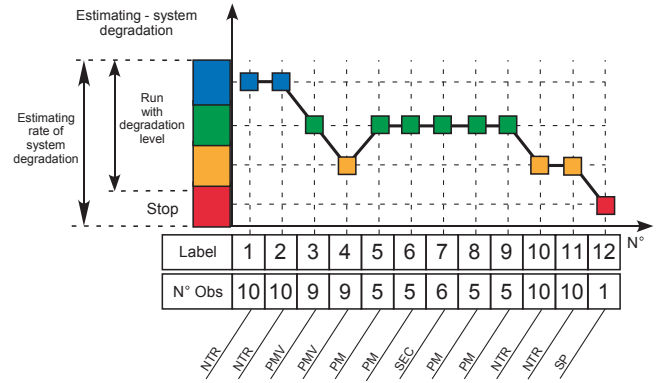
Fig. 2. Example of a degradation sequence of a process. The process starts at level 4. It becomes more and more degraded over time. After a Preventive Maintenance Visit (PMV), you can see that the degradation level increases on level 3. It decreases again until nothing is done (NTR: Nothing To Report) see label 10 and 11. Then, the process stops on label 12 (SP). PM is the symbol for Preventive Maintenance and SEC for a Security report.
