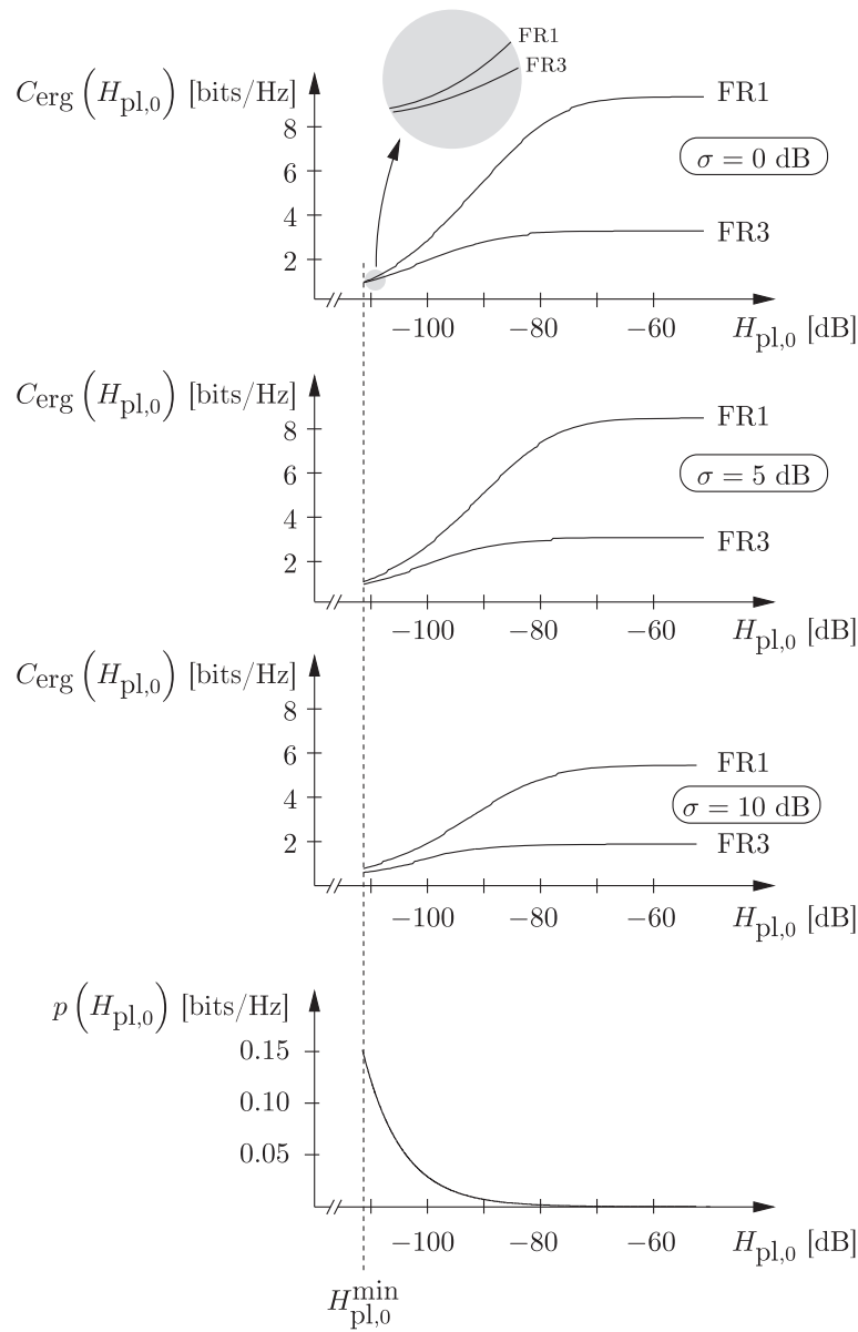
Figure 6 Plots of the ergodic capacities C_{erg}^{wf,FR1} and C_{erg}^{wf,FR3} as functions of the path loss H_{pl,0} of the typical user UT_0 for several values of the shadowing standard deviation: \sigma_{dB} = 0, 5 and 10 dB (full-CSI scheme). The FR1 pattern performs better than the FR3 pattern, for the whole [0, 10] -dB range of values of \sigma_{dB} .
