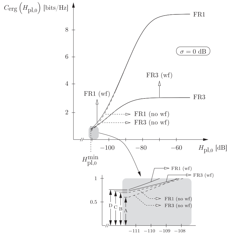
Figure 7 We illustrate the waterfilling gain for the ergodic capacity at the minimum path loss H_{\text{pl},0}^{\min} for both frequency reuse schemes FR1 and FR3 (full-CSI scheme). We see from the bottom figure that C/A > D/B , which results from (24).
