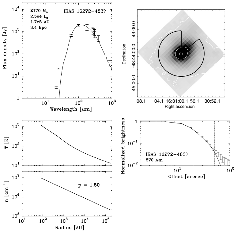
Fig. C.2. As Fig. C.1, for IRAS 16272.
