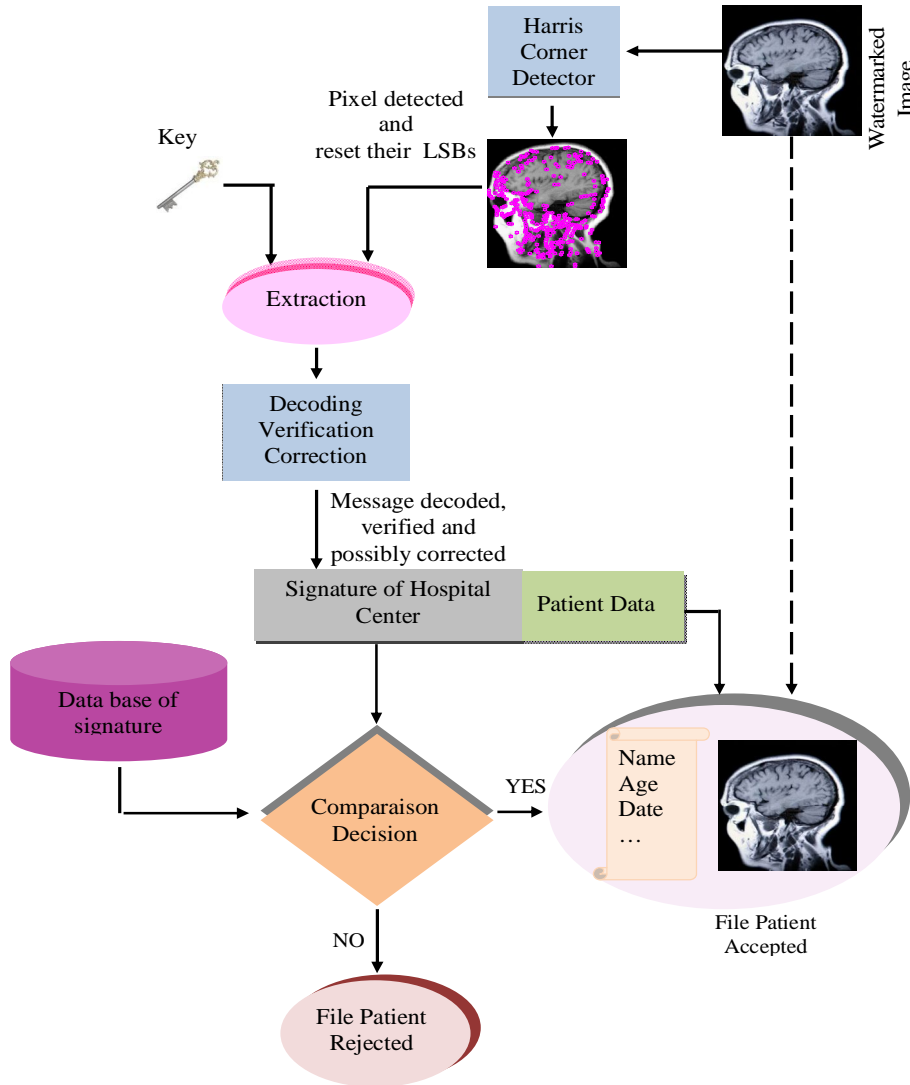
Fig. 5. Watermarked extraction algorithm.
