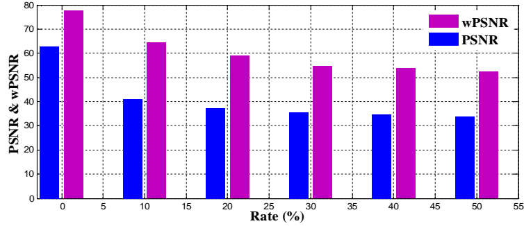
Fig. 7. PSNR and wPSNR for IRM image watermarked compressed.
