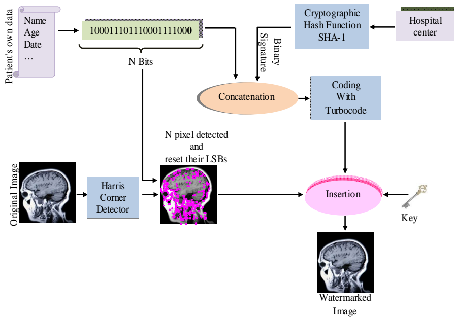
Fig. 4. Watermarked insertion algorithm.
