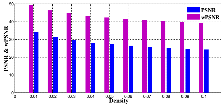
Fig. 9. PSNR and wPSNR for Echographic images watermarked and attacked by an impulsionnel noise.
