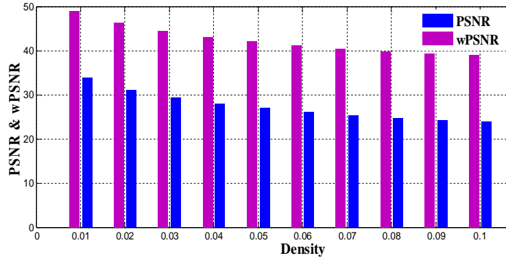
Fig. 10. PSNR and wPSNR for IRM images watermarked and attacked by an impulsionnel noise.
