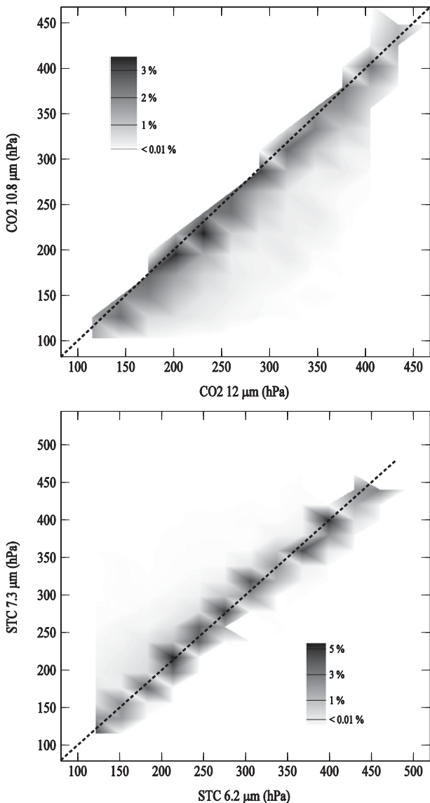
FIG. 5. Density plots of (top) CO 2 10.8 pressure vs CO 2 12 pressure and (bottom) STC7.3 pressure vs STC6.2 pressure. The gray scale represents the dot density, given in percent of the total number of ice clouds simulations.
