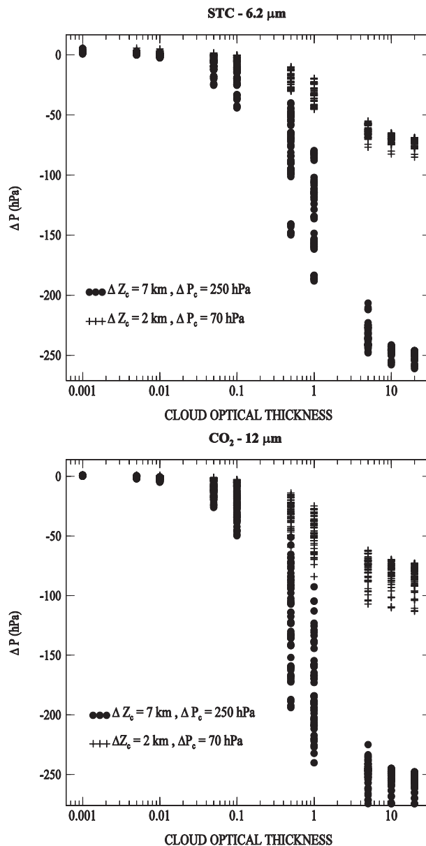
FIG. 6. Multilayer situations for which thin cirrus clouds are above a lower cloudy layer located 2 km (plus signs) and 7 km (filled circles) below. Pressure difference \Delta P defined as the difference between the retrieved pressure and the pressure set to the top of the lowest layer in the simulation, is presented as a function of the upper cirrus optical thickness.
