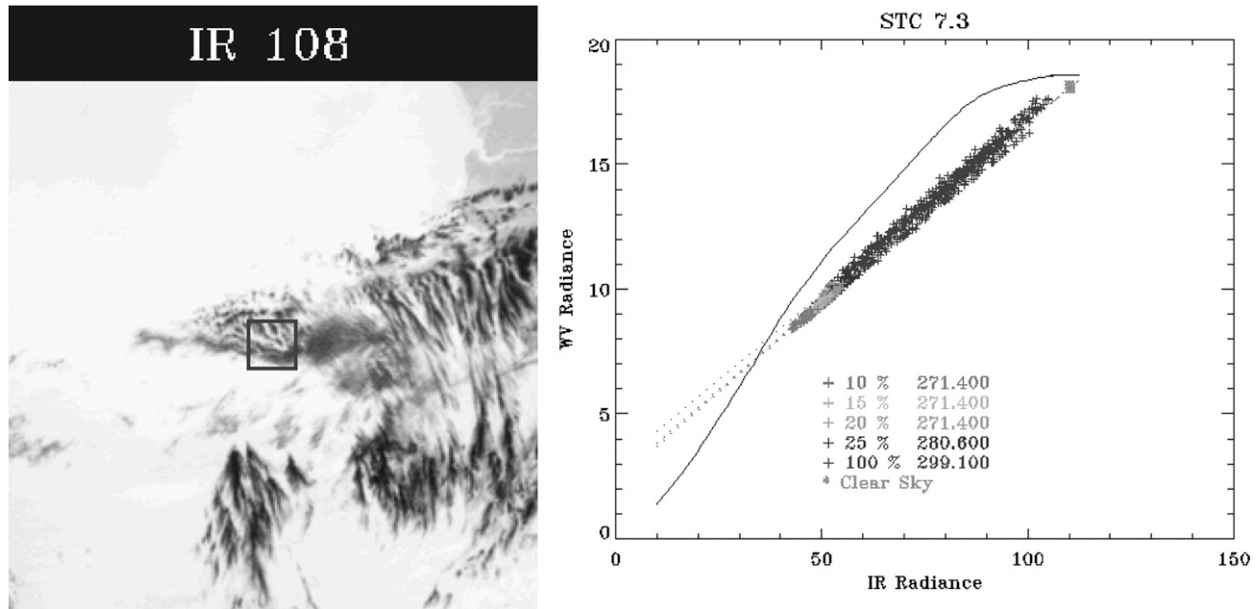
FIG. 1. Examples of the STC method that uses channels IR10.8 and WV7.3 applied to the 24 \times 24 pixels target area illustrated in the Meteosat image on the left (taken at 0230 UTC 1 Dec 2002, at 10.5^{\circ}\text{N} , 19.66^{\circ}\text{E} ). The different pressures have been retrieved using 10%, 15%, 20%, 25%, and 100% of the coldest cloudy pixels (in black on the image) present within the target area. The black solid curve represents the WV7.3 and IR10.8 radiances as calculated by a radiative transfer model for an opaque cloud at various pressure levels in the atmosphere.
