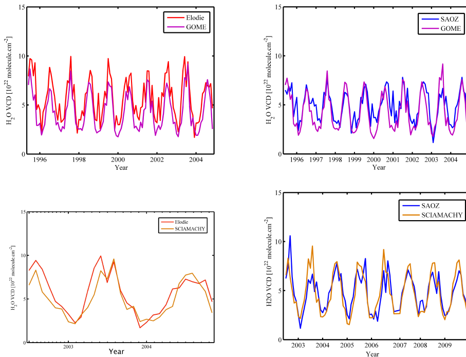
Fig. 4. Comparison of monthly average of \text{H}_2\text{O} obtained by ground-based SAOZ, Elodie and satellites GOME, SCIAMACHY above OHP.
