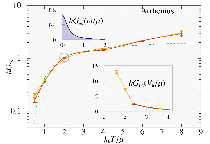
Figure 3: Finite-temperature, zero-frequency longitudinal conductance for an intensity of the disorder V_R = 2.4 \mu . Error bars refer to averages over disorder and the dashed line is a fit to a simple exponential Arrhenius law G_{\text{DC}}(T) \propto e^{-\frac{AE}{k_B T}} . In the upper inset, the complete frequency dependence of the conductance is exemplified for k_B T = 2\mu . In the lower inset, the conductance at constant temperature ( k_B T = \mu ) and varying disorder strength is also shown. In all cases darker curves mark increasingly large sizes, in the range L/\sigma_R = 20 - 40 .
