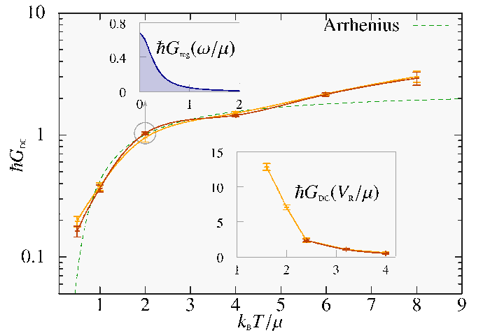
Figure 3: Finite-temperature, zero-frequency longitudinal conductance for an intensity of the disorder V_R = 2.4 \mu . Error bars refer to averages over disorder and the dashed line is a fit to a simple exponential Arrhenius law G_{\text{DC}}(T) \propto e^{-\frac{AE}{k_B T}} . In the upper inset, the complete frequency dependence of the conductance is exemplified for k_B T = 2\mu . In the lower inset, the conductance at constant temperature ( k_B T = \mu ) and varying disorder strength is also shown. In all cases darker curves mark increasingly large sizes, in the range L/\sigma_R = 20 - 40 .
