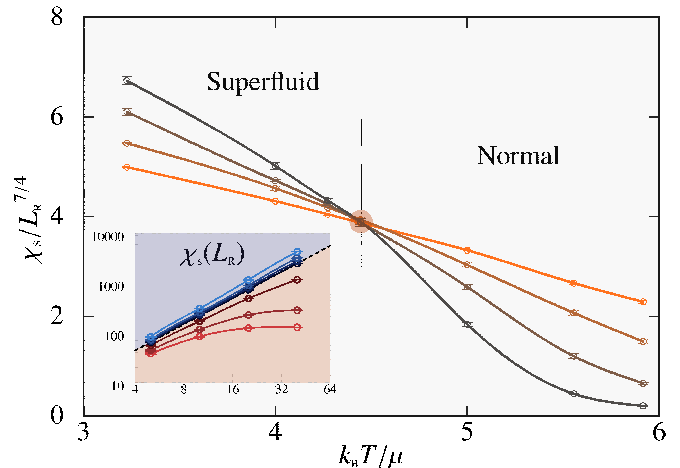
Figure 1: Scaled superfluid susceptibility against temperature for system sizes ranging from L_R = L/\sigma_R = 5 - 40 at disorder strength V_R/\mu = 0.3 and interaction strength \tilde{g} = 0.1 . Darker curves mark increasingly large size. In the inset, the susceptibility is shown as a function of L_R (temperature increases from top to bottom). The divergence predicted by the BKT transition for clean systems ( \eta = 1/4 ) is indicated by the dashed line.
