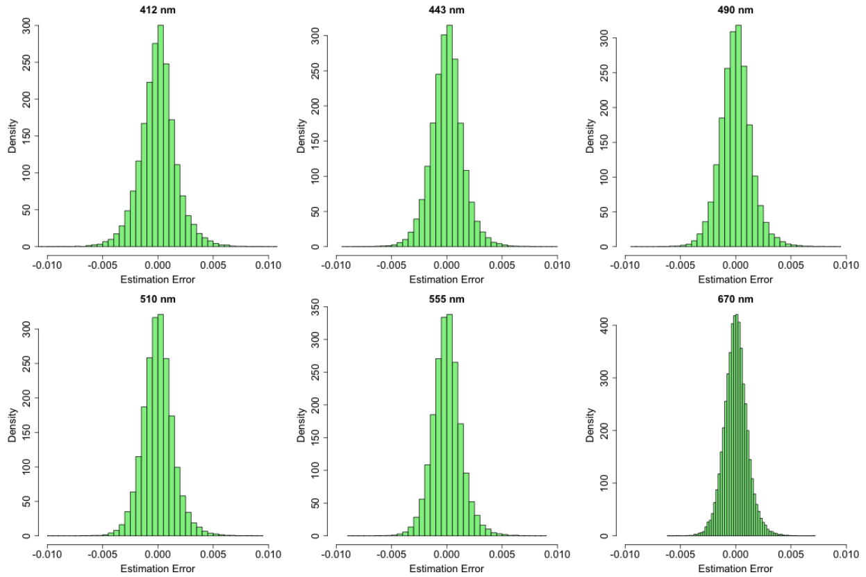
Figure 20: Histograms of \rho_a estimation error.
