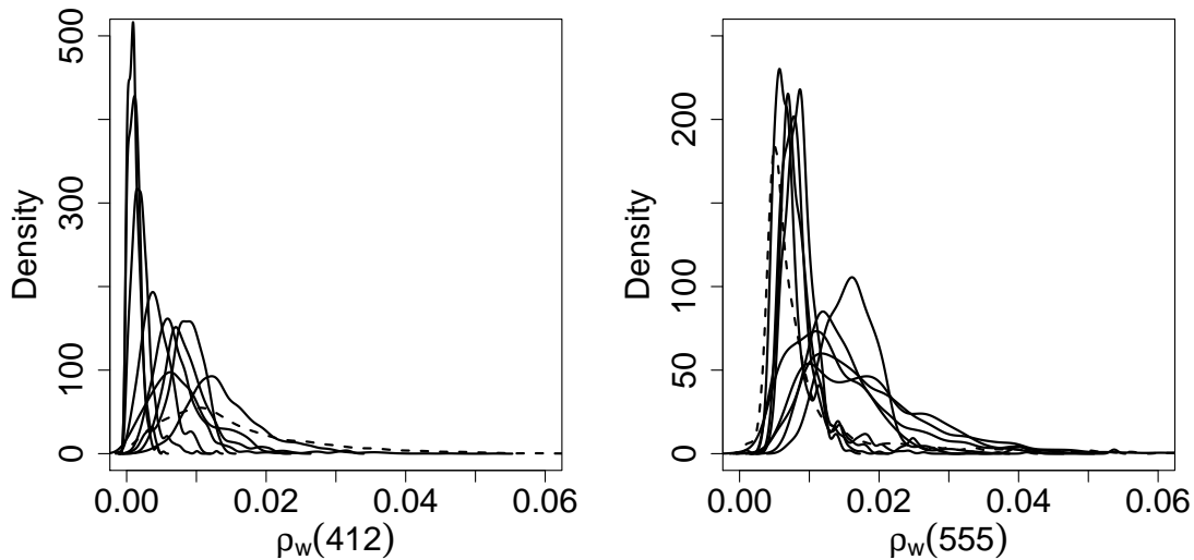
Figure 4: Estimated densities of the marine reflectance at 412 and 555 nm, left and right, respectively, acquired at each of the 9 AERONET sites (solid lines) and assembled in NOMAD (dashed line).
