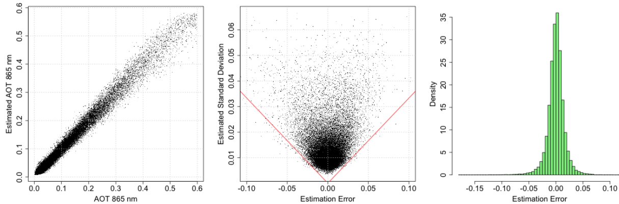
Figure 18: (Left) Estimated versus simulated \tau_a . (Center) Estimated standard \tau_a standard deviation versus \tau_a estimation error with lines of slopes \pm 1/3 . (Right) histogram of \tau_a estimation errors.
