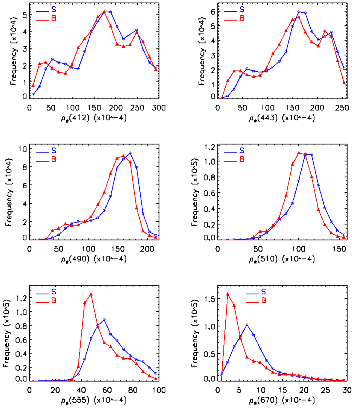
Figure 26: Histograms of valid \rho_w estimates obtained with the Bayesian technique (B) and the SeaDAS algorithm (S). The Bayesian estimates are shifted toward lower values.
