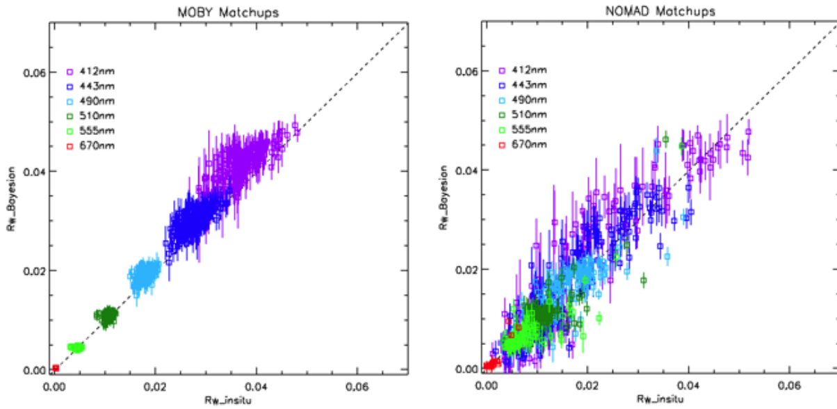
Figure 34: Estimated versus measured marine reflectance for MOBY and NOMAD match-up data sets.
