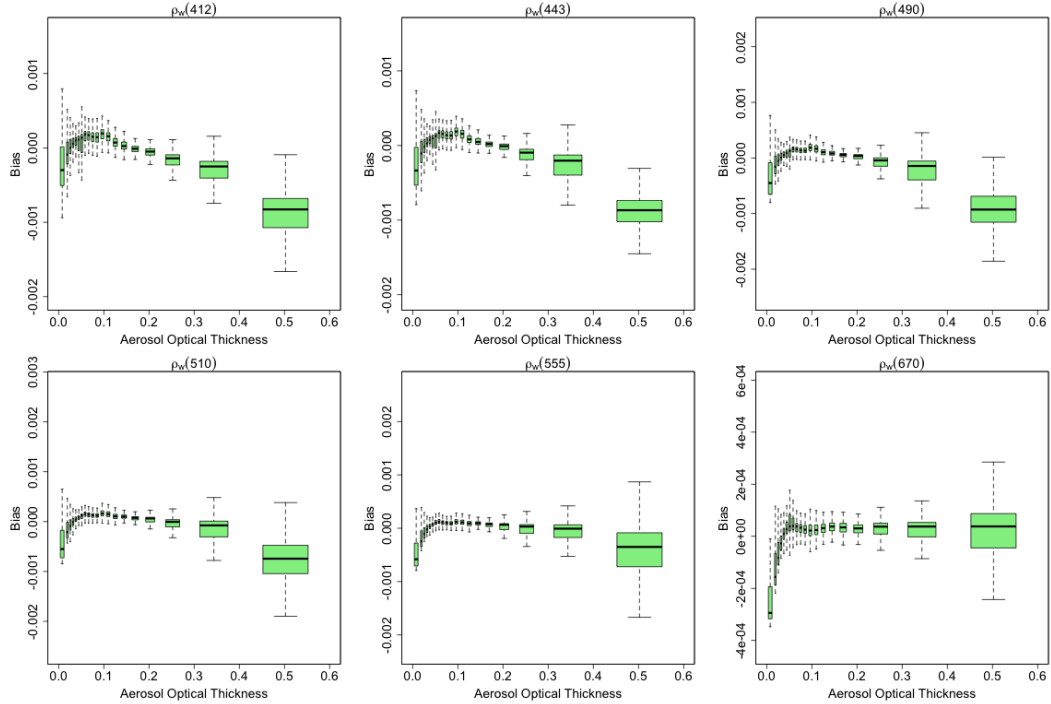
Figure 11: Bias per spectral band and aerosol optical thickness bin, with all the geometries.
