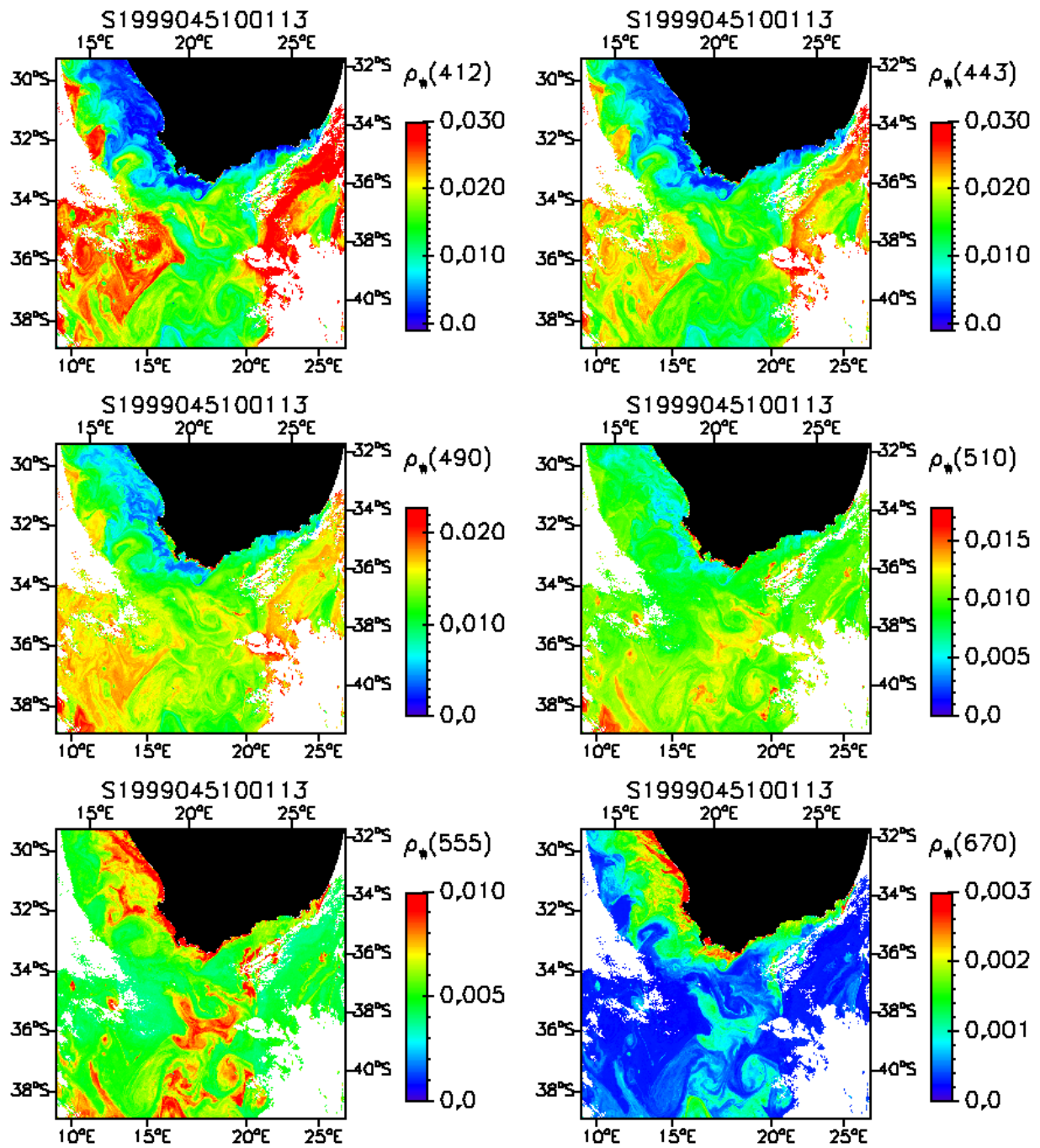
Figure 23: Estimated \rho_w by the Bayesian methodology.
