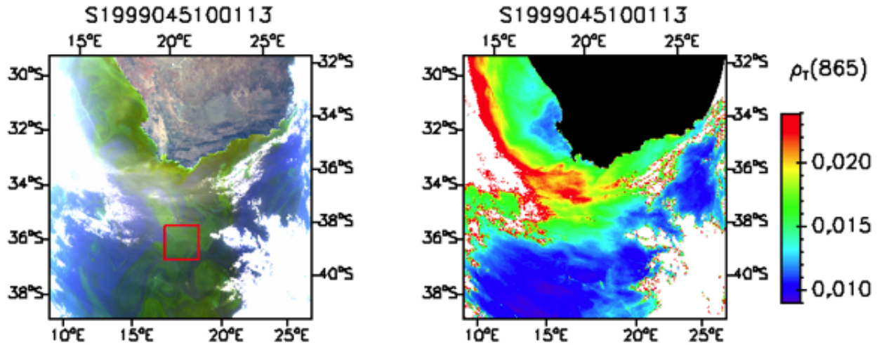
Figure 22: SeaWiFS imagery of the ocean off South Africa acquired on February 14, 1999. Left: True color image. Right: TOA reflectance at 865 nm. Clouds are masked in white according to SeaDAS.
