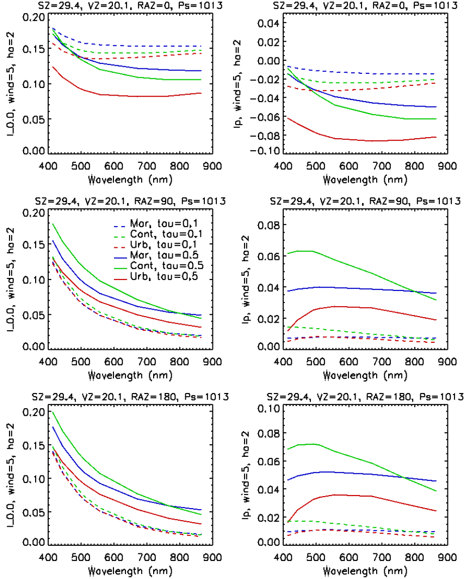
Figure 2: Simulations of the top-of-atmosphere normalized radiance ( \pi L_{toa}/F_s ) by a vector radiation transfer code based on the successive-orders-of-scattering method. The atmosphere contains molecules and aerosols and is bounded by a wavy surface. Backscattering by the water body is null. Sun zenith angle is 29.4 deg., view zenith angle is 20.1 deg., relative azimuth angle is 0 (top panels), 90 deg. (middle panels), and 180 deg. (bottom panels), wind speed is 5 m/s, and surface pressure is 1013 hPa. Three types of aerosols are considered, i.e., maritime, continental, and urban, and aerosol optical thickness is 0.1 and 0.5 at 865 nm. Aerosol scale height is 2 km. The total signal is displayed in the left panels, and the signal after subtraction of the molecular signal (calculated assuming no aerosols) is displayed in the right panels.
