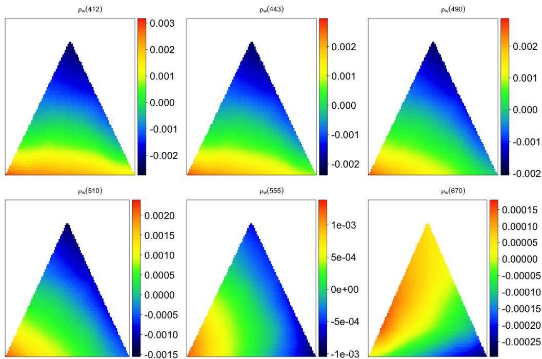
Figure 13: Bias per spectral band, averaged over all geometries, as a function of the aerosol type.
