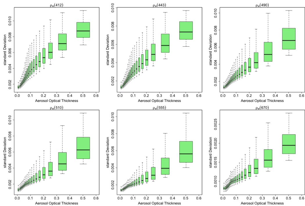
Figure 12: Standard deviation per spectral band and aerosol optical thickness bin, with all the geometries.
