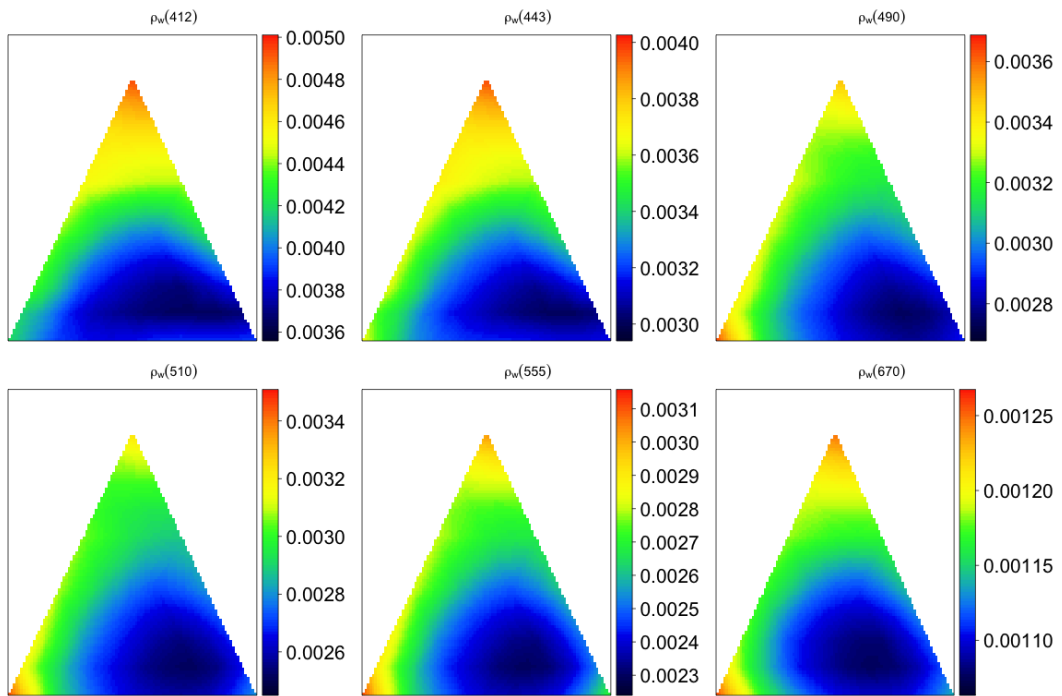
Figure 14: Standard deviation per spectral band, averaged over all geometries, as a function of the aerosol type.
