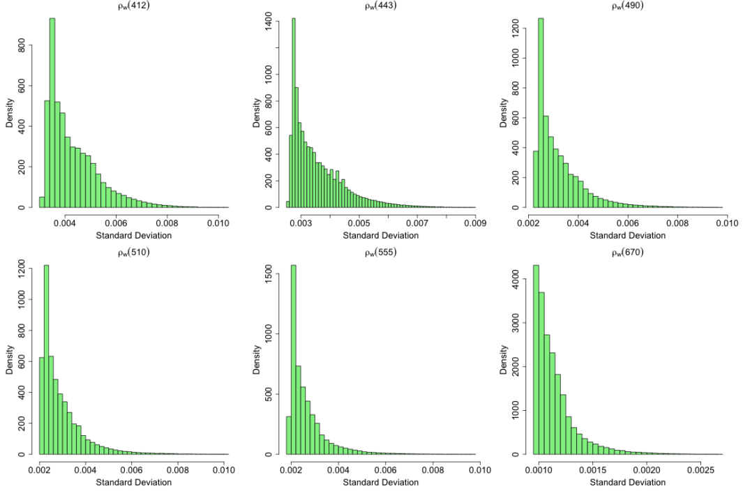
Figure 7: Global statistics: histograms of the standard deviation per wavelength.
