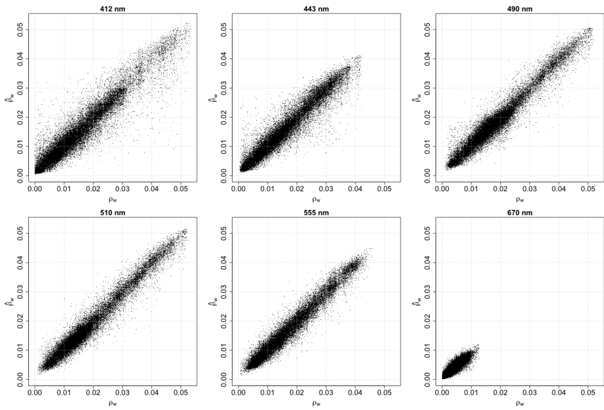
Figure 15: Estimated versus simulated \rho_w .
