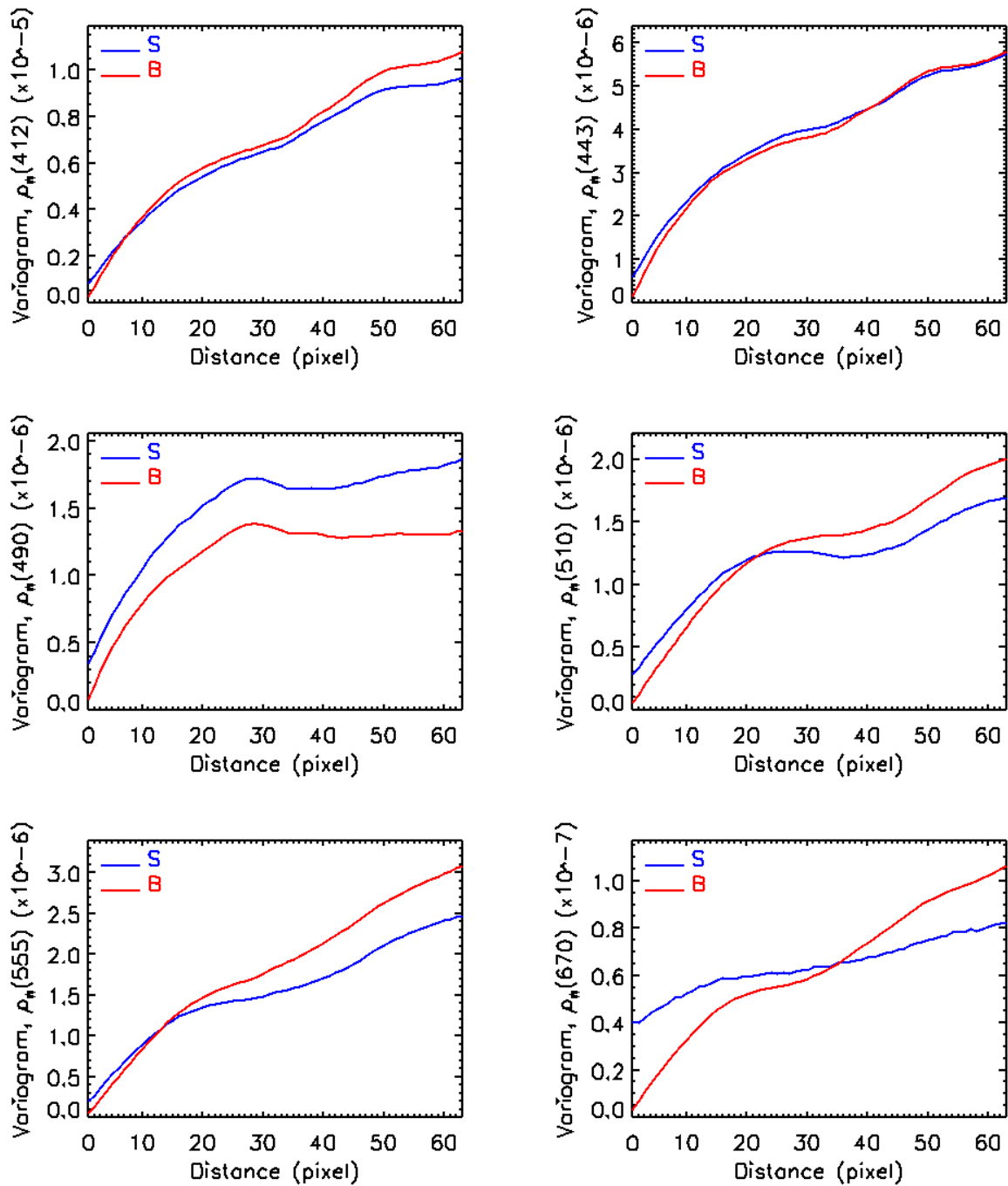
Figure 27: Variograms of valid \rho_w estimates obtained with the Bayesian technique (B) and the SeaDAS algorithm (S). Computations are made using data in a 128x128 pixel area South of the Cape of Good Hope. The variograms obtained with the statistical method indicate less noisy retrievals.
