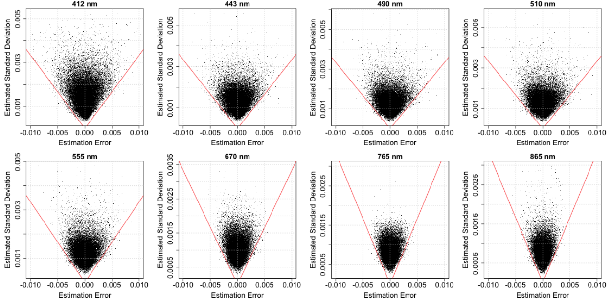
Figure 21: Estimated \rho_a standard deviation versus \rho_a estimation error, with lines of slopes \pm 1/3 .
