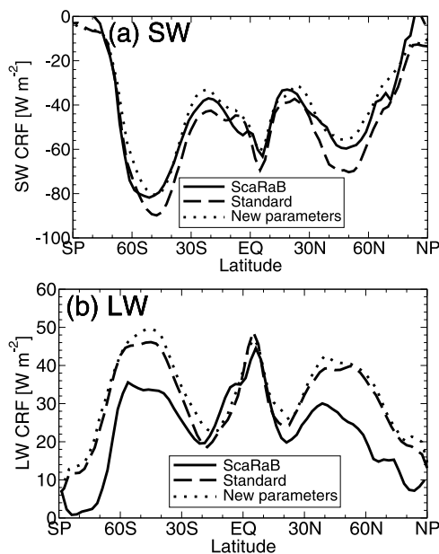
Figure 7. Annually-averaged cloud radiative forcing in the (a) short-wave and (b) long-wave spectrum for ScaRaB observations (solid), the standard model scheme (dashed), and the new pair of parameters (dotted).
