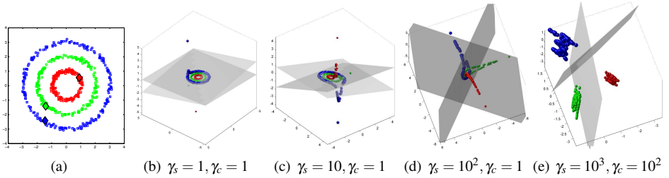
Figure 1: (a) This figure shows the input data where different colors stand for different classes; red-colored data are annotated with (1 \ -1)' , blue-colored data with (-1 \ 1)' and green-colored data with (1 \ 1)' . Note that just one training sample per class (diamond-shaped) is labeled while others are unlabeled. Our algorithm is initialized with p = 10 and after 5 iterations (before convergence) it reduces the ranks to 4. Figures (b,c,d) are the learned kernel maps (shown in 3d) and the obtained decision hyperplanes for different setting of the parameters \gamma_c and \gamma_s .
