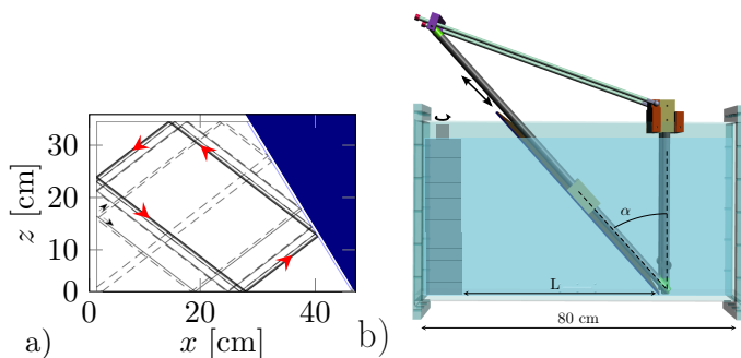
FIG. 1. (Color online) Panel (a) presents the prediction of a wave-ray billiard with a bottom length L = 45.6 cm and a depth H = 32.6 cm, while the sloping wall is inclined at an angle \alpha = 30^\circ with the vertical. The ray direction (defined by the group velocity) of the limit-cycle is counter-clockwise as shown by red arrows. Panel (b): Corresponding experimental setup showing the wave generator and the sloping wall inside the immobile tank of size 80 \times 17 \times 42.5 cm. The working bottom length of the section, the depth and the sloping angle are the one given in panel (a). Conventional double-bucket technique is used to create a uniform stratification with a buoyancy frequency N = 0.95 rad/s.
