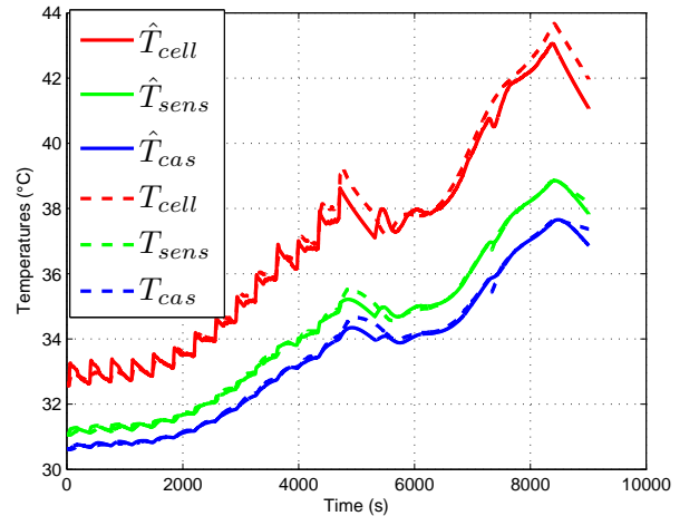
Figure 8: Real and estimated temperatures (constant gain, \sigma = 7.8 ).
