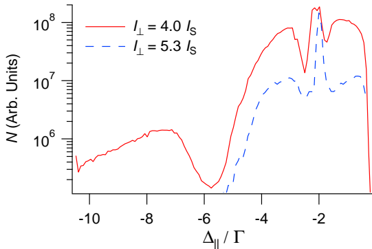
Figure 3. Number N of atoms in the cloud versus \Delta_{\parallel} for \Delta_{\perp} = -2\Gamma , I_{\parallel} \simeq 9I_S and different values of I_{\perp} .
