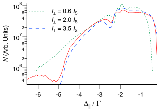
Figure 2. Number N of atoms in the cloud versus \Delta_{\parallel} for \Delta_{\perp} = -2\Gamma , I_{\parallel} \simeq 2I_S and different values of I_{\perp} .
