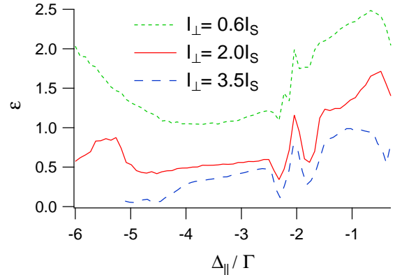
Figure 4. Ellipticity \varepsilon of the atomic cloud versus \Delta_{\parallel} for \Delta_{\perp} = -2\Gamma , I_{\parallel} \simeq 2I_S and different values of I_{\perp} .
