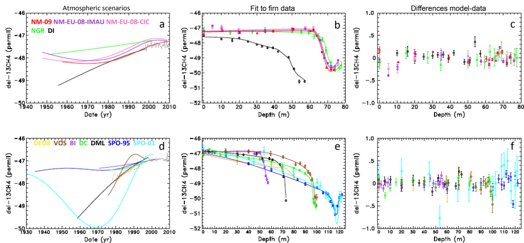
Fig. 2. Single site \delta^{13}\text{C}(\text{CH}_4) trend scenarios ( a,d ), the fit to the firn data ( b,e ) and model-data differences ( c,f ). NH sites ( a–c ). SH sites ( d–f ). The site names and color codes are as given in the legend of Fig. 1. The grey curve ( a,d ) represents air-archive from Cape Grim (Francey et al., 1998) and continuous atmospheric monitoring data from the NOAA-ESRL network.
