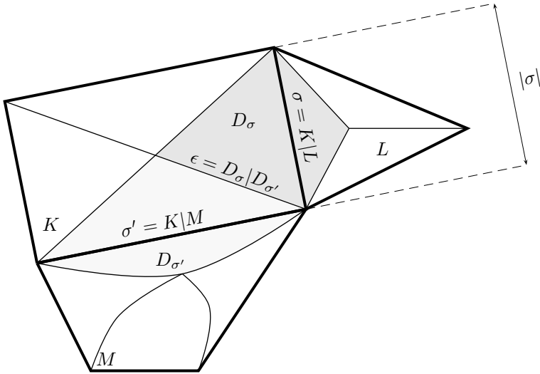
FIG. 2.1. Primal and dual meshes for the Rannacher-Turek and Crouzeix-Raviart elements.
