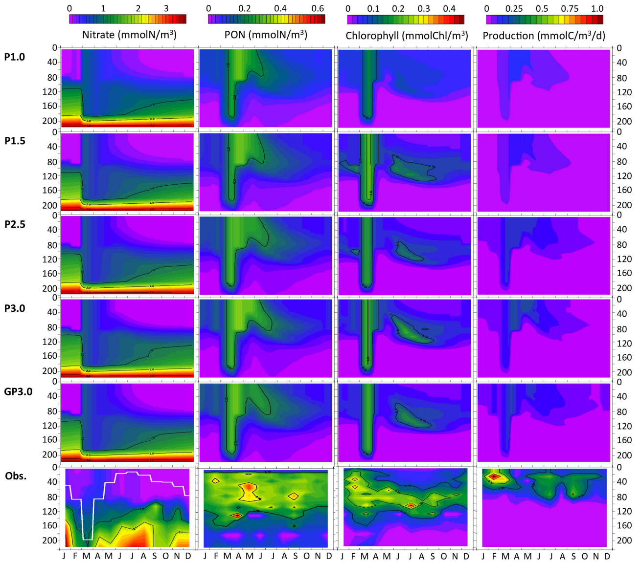
Figure 4: Seasonal cycles of nitrate, particulate organic nitrogen (PON), chlorophyll, and primary production at BATS in 1998, simulated with the different models after optimization and observed at BATS in 1998. The observed mixed layer depth is superimposed in white over the observed nitrate profiles.
