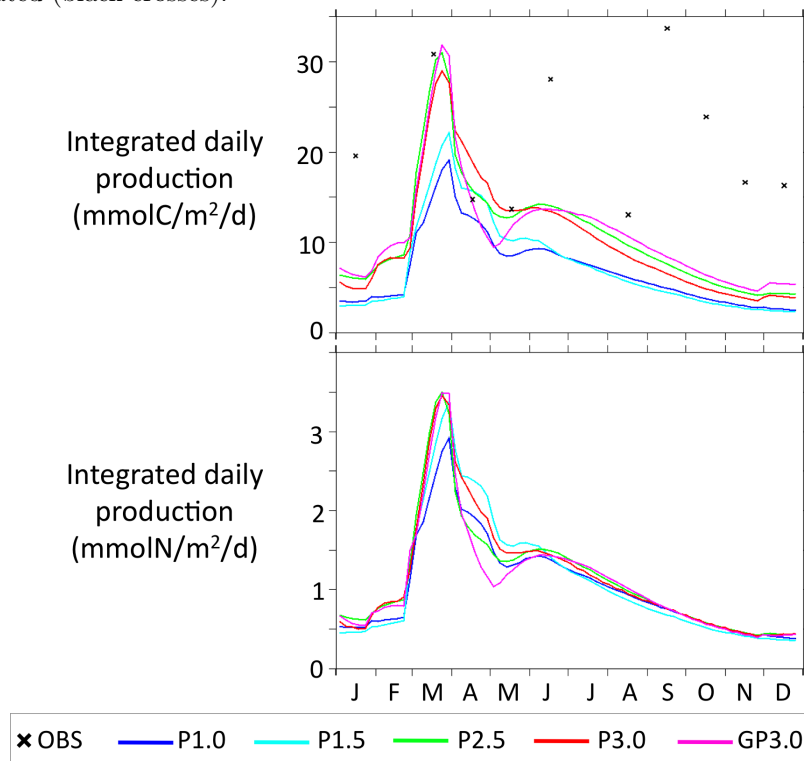
Figure 6: Temporal evolution of integrated daily production in carbon and in nitrogen from 0 to 234 m, simulated by the Redfield formulations P1.0 (blue) and P1.5 (light blue), and by the quota formulations P2.5 (green), P3.0 (red), and GP3.0 (magenta) after optimization. The observed values of the integrated daily production in carbon at BATS are indicated (black crosses).
