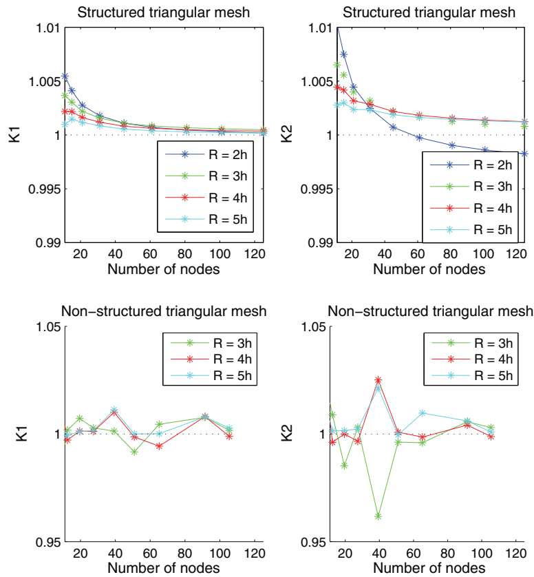
Figure 10. Stress intensity factors calculations—Direct estimate—First test case—Triangular meshes.
