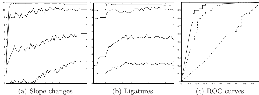
Fig. 3. Resistance to spurious slope changes (a) and spurious branches(b). For (a) and (b) the kernels are from top to bottom: K_{change,edit2} (—), K_{change,edit1} (—|—), random walk kernel(---), and K_{change,classic} (-·-). (c) ROC curves for the classification of dogs and cats using: K_{change,edit} (—), random walk kernel (---) and K_{change,classic} (-·-).
